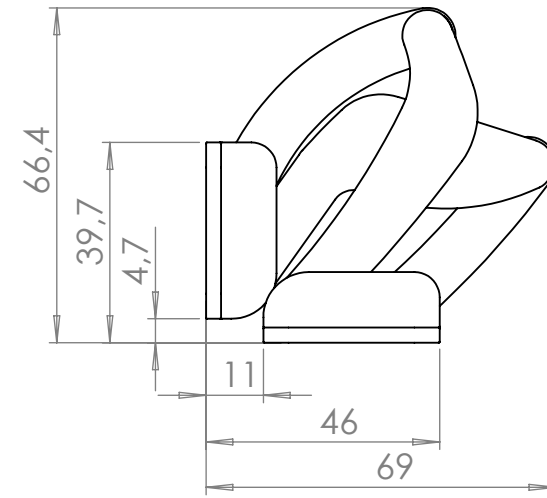
Compact spiderhinge, 0°
