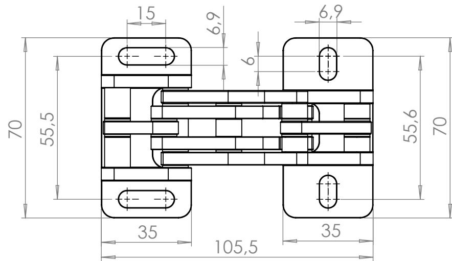
Compact spider hinge, 90° (Top view)
