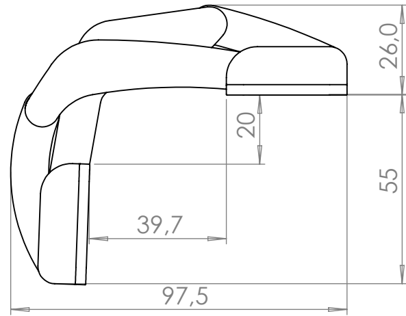
Compact spider hinge, 178° (Maximum opening)
